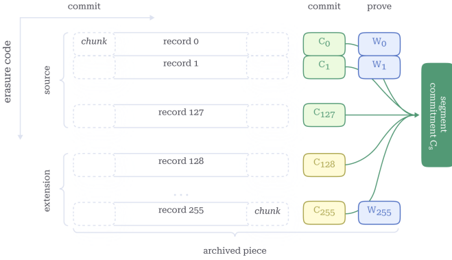
Fig. 5. Archived segment
