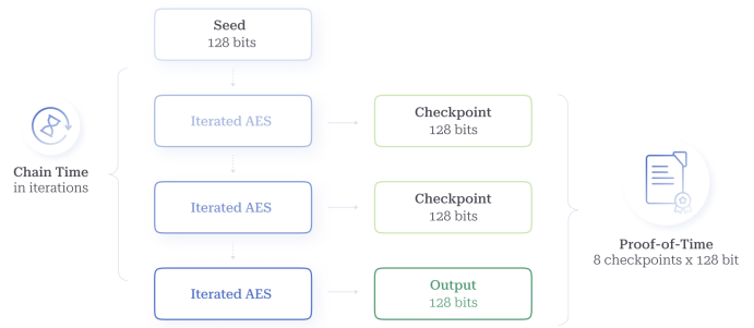
Fig. 7. Proof-of-Time checkpoints
